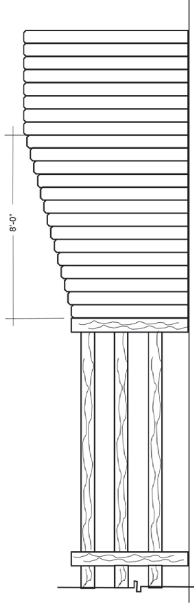
6' PRIVACY FENCE TRANSITION PANEL TO 3 RAIL FENCE.
